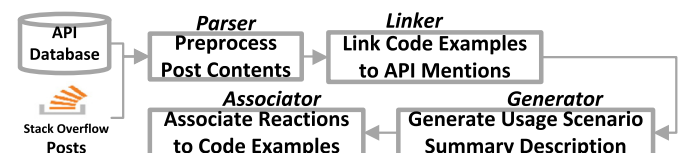
Fig. 3. The major components of our API usage scenario mining framework.
