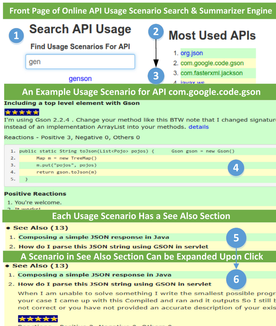
Fig. 9. Screenshots of online our task-based API documentation tool.
