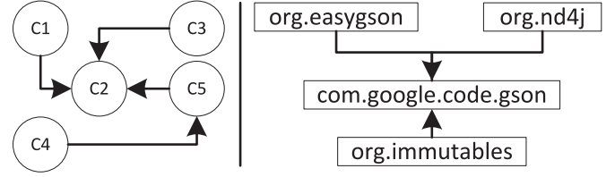
Fig. 7. Dependency graph given a hit list.
