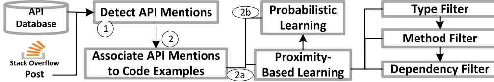
Fig. 5. The components to link a scenario to API mention.
