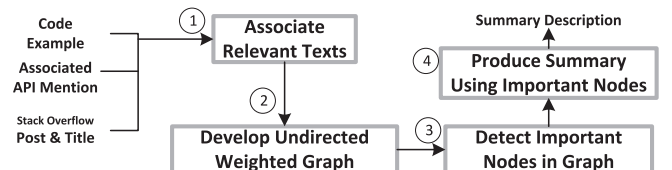
Fig. 8. Steps to produce summary description of a scenario.
