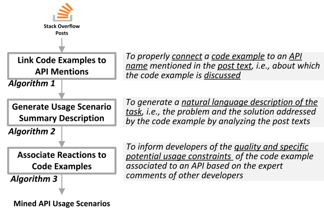
Fig. 1. Our API usage scenario mining framework from Stack Overflow with three proposed algorithms.
