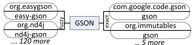
Fig. 6. Partial Mention Candidate List of GSON in Figure 2.
